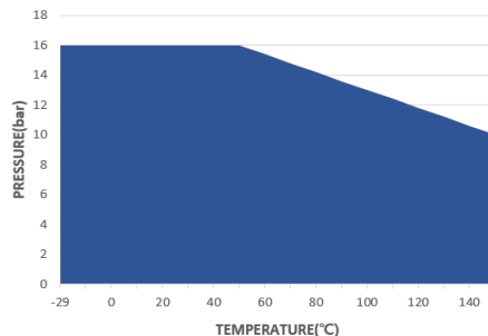
Pressure-Temperature Chart
